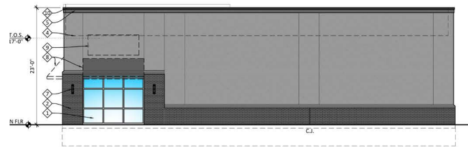
PRELIMINARY EAST ELEVATION SCALE: 1/8" = 1'-0" 5
