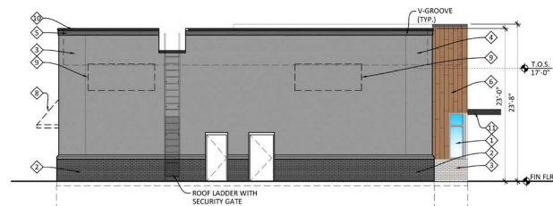
PRELIMINARY WEST ELEVATION SCALE: 1/8" = 1'-0" 3
